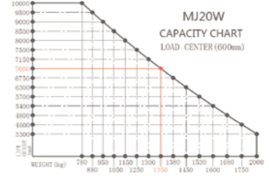
Capacity Chart -MJ20W
