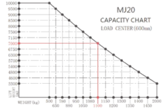
Capacity Chart-MJ20
