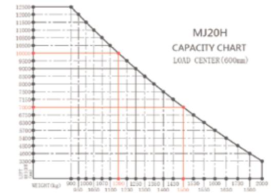
Capacity Chart-MJ20H
